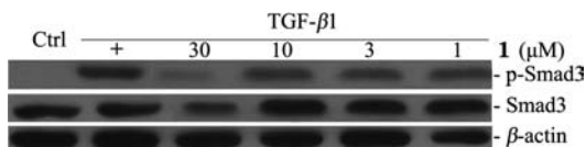
Figure 3. Compound 1 blocks TGF- \beta 1-mediated Smad3 phosphorylation in a dose-dependent manner. NRK 52E cells were treated with TGF- \beta 1 (10 ng/mL) for 1 h in the absence or presence of different doses of compound 1 as indicated. Ctrl: untreated cells.
