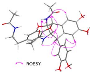
Figure 2. Important ROESY correlations of ( \pm )-1.
