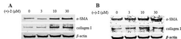
Figure 4. Compound (+)-2 (A) or (–)-2 (B) upregulates \alpha -SMA and collagen I in a dose-dependent manner. NRK 52E cells were treated with (+)-2 or (–)-2 for 48 h at doses of 3, 10, and 30 \mu M as indicated. Cell lysates were immunoblotted with antibodies against \alpha -SMA and collagen I. Data are expressed as mean \pm SD. ANOVA, * p < 0.01 vs control. Ctrl: untreated cells.
