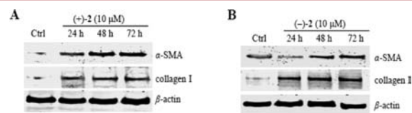
Figure 5. Compound (+)-2 (A) or (–)-2 (B) upregulates \alpha -SMA and collagen I in a time-dependent manner. NRK 52E cells were treated with (+)-2 or (–)-2 at the dose of 10 \mu M for 24, 48, and 72 h as indicated. Western blot analyses were used to test the protein expression of \alpha -SMA and collagen I. Data are expressed as mean \pm SD. ANOVA, * p < 0.01 vs control. Ctrl: untreated cells.
